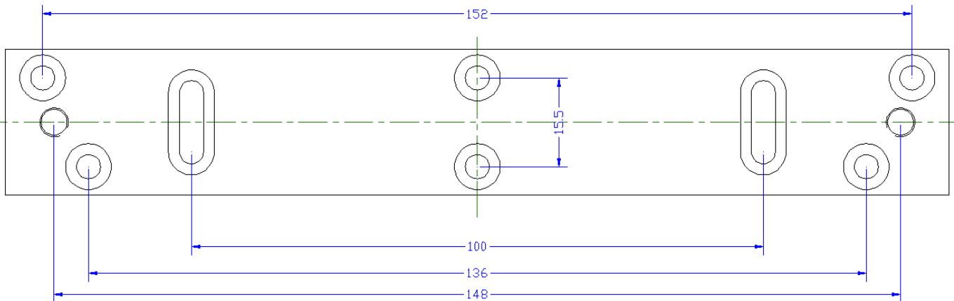
SETTLEMENT PLATE DIMENSION
